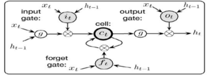
Fig. 2. The diagram of LSTM Block.
