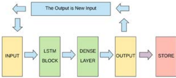
Fig. 1. The network architecture for the recursive forecasting
